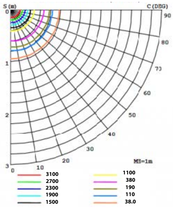
PLANAR ISOLUX DIAGRAM (UNIT: 1x)
